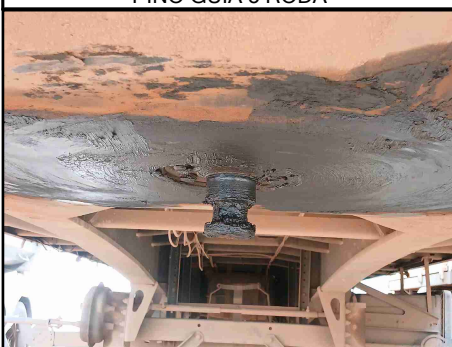
PINO GUIA 5 RODA
